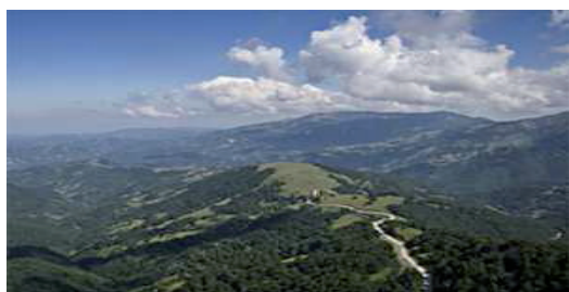
Fig.3.5. Midžor peak: A- CORINE Land Cover 2000, B-satellite imagery, C-image. (Red arrows indicate areas of class 324)
