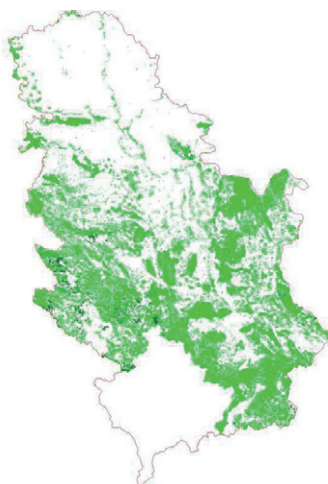
Fig.3.8. Forest land, CORINE Land Cover 2000.
