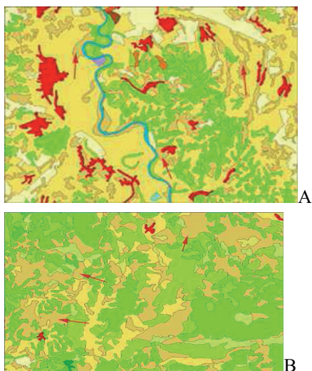
Fig.3.6. Class 243, CORINE Land Cover 2000th. A- near river Morava, B-in high mountain areas. Red arrows indicate areas of class 243.
